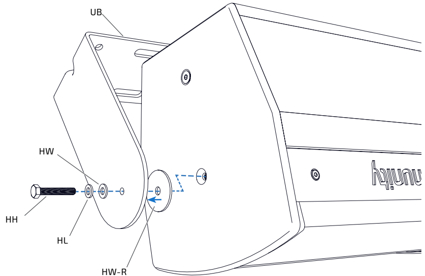
Figure 1. Remove middle cabinet bolts and attach yoke to cabinet
