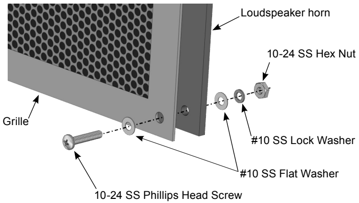
Figure 2. Grille installation ( RMG-200A shown)
