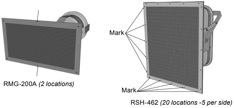
Figure 1. Place grille on horn, align edges, and mark holes
