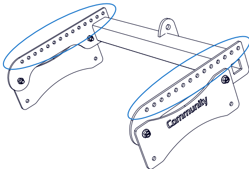
Connect suspension hardware to upper holes along the side rails (circled) Use defined Pin# from EF3
