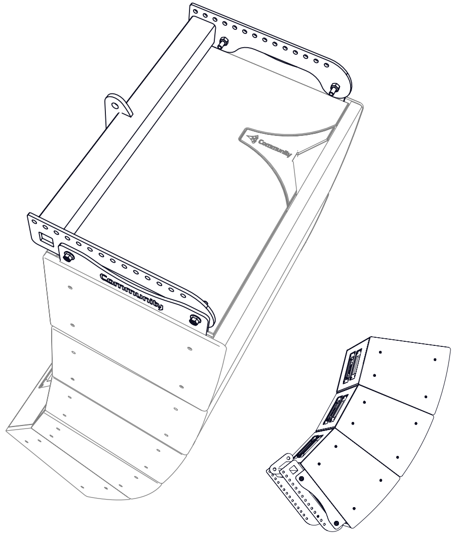
IV6 Light Array Frame / Pull Back Bar (shown with loudspeakers)
