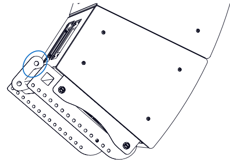
Connect pullback cable hardware to the upper hole of the center tab (circled) welded to the square tube
