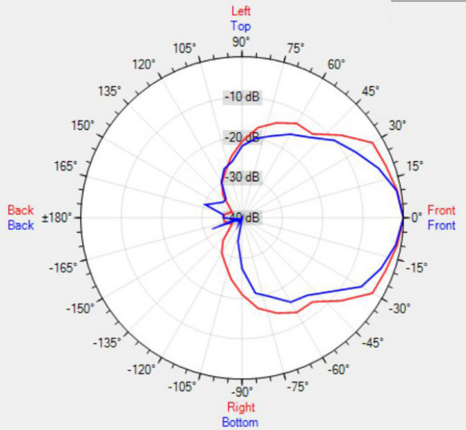
Data Shown: MASK12T-90x70 (Apart Audio) Display Parameters: Frequency: 8000Hz (1/24th Octave)
