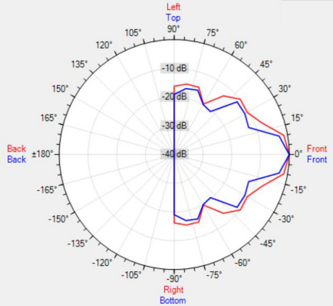
Data Shown: EN-SMS6T6-W (APart Audio) Display Parameters: Frequency: 8000Hz (1/24th Octave)
