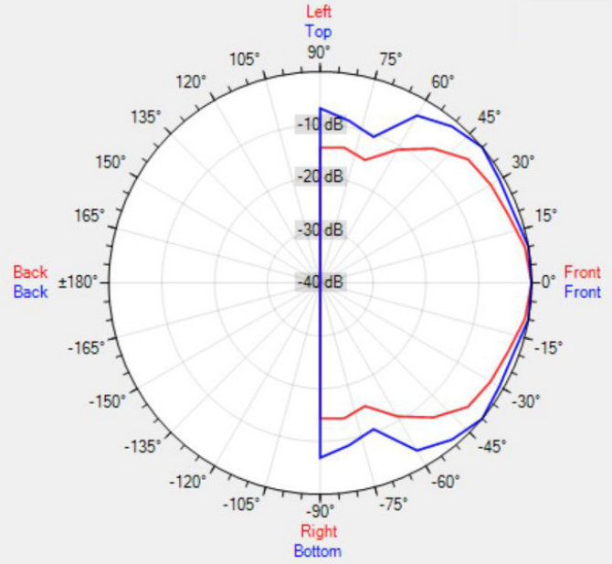
Data Shown: EN-SMS6T6-W (APart Audio) Display Parameters: Frequency: 2000Hz (1/24th Octave)
