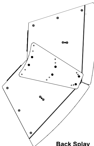
Back Splay 0° hole set
