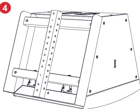
Array frame attached
