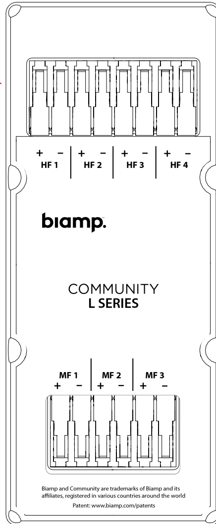
MF/HF Input Panel LVH-900/AP
