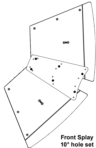
Figure 4. Typical splay bracket orientation - cabinet connection locations are symmetrical on the splay bracket
