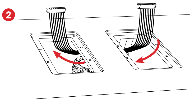
Figure 10. Thread harness through openings
