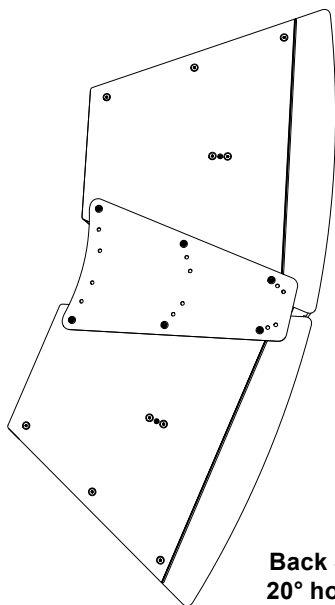
Figure 4. Typical splay bracket orientation - cabinet connection locations are symmetrical on the splay bracket
