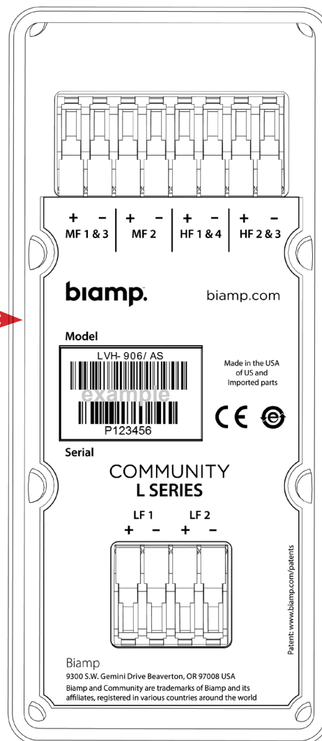
Input Panel LVH-900/AS
