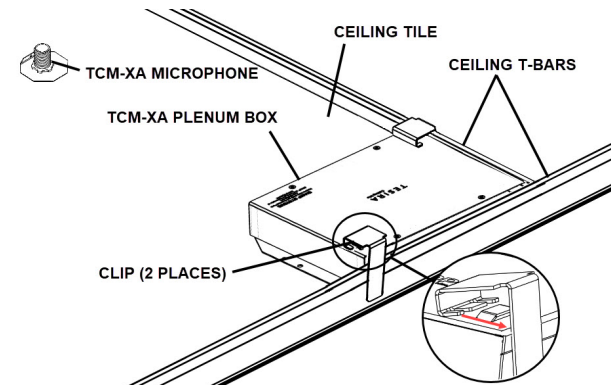
Figure 8. Above-Ceiling Tile Corner Installation Option
