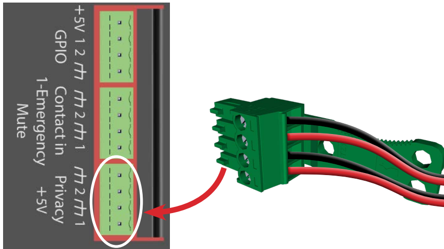
Figure 9. Privacy lights connection / wiring
