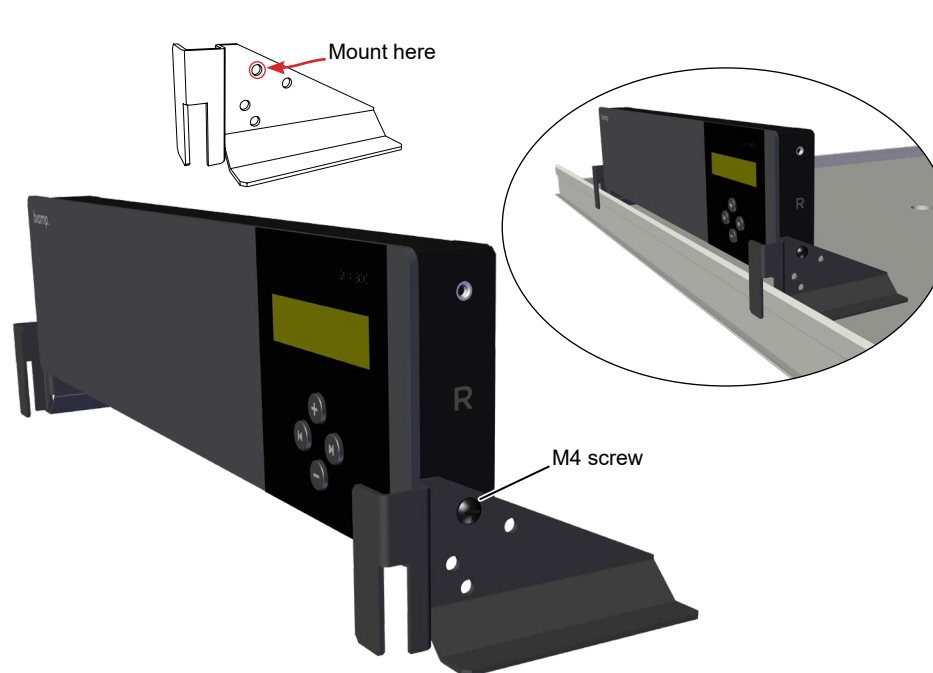
Figure 40. Controller is raised above the rail
