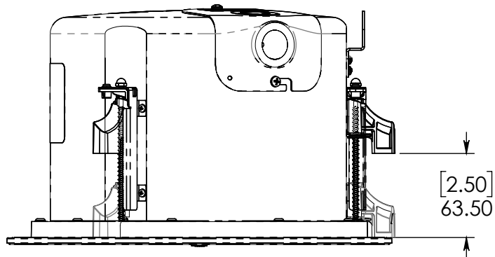
MOUNTING DOG GRIP RANGE DETAIL (DOGS SHOWN IN MAX AND MIN POSITION)
